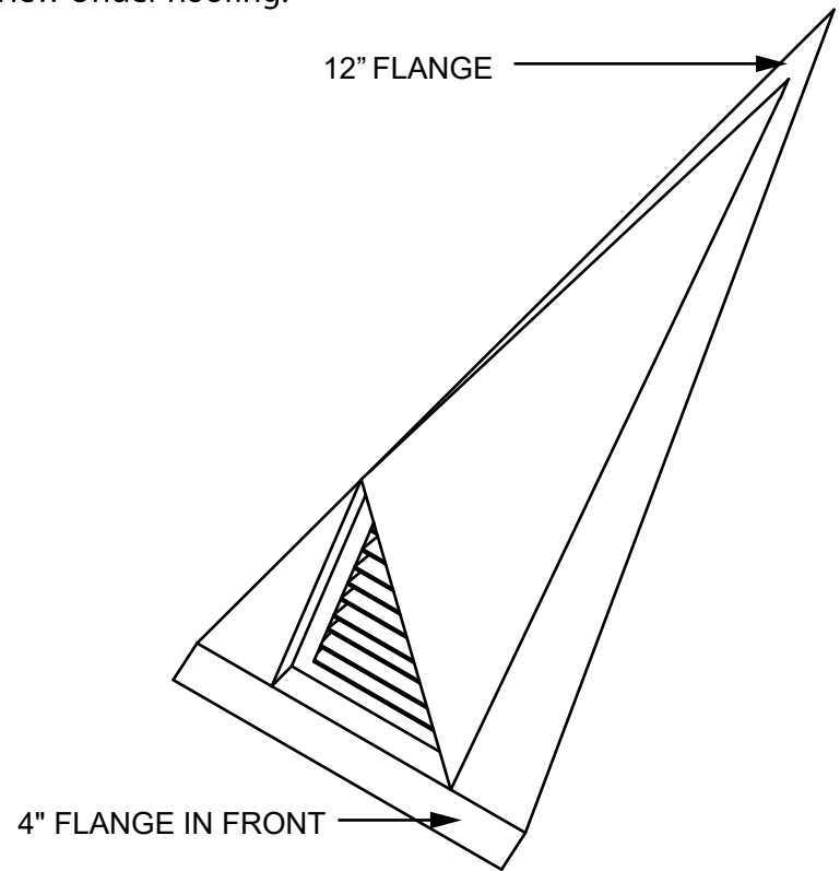
Isometric View Under Roofing:
